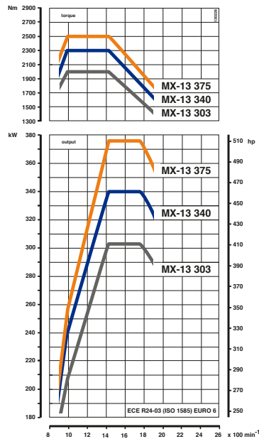
PACCAR MX-13
